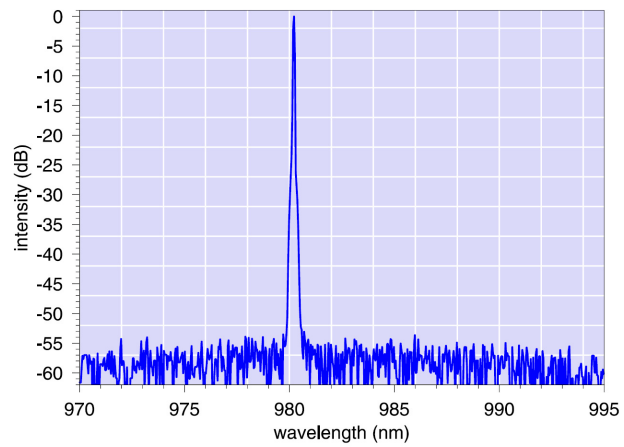
Room Temperature CW Spectrum at 980nm
